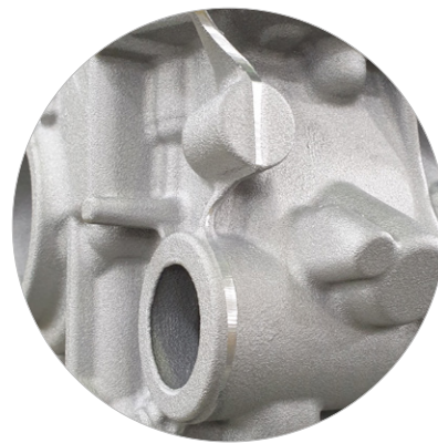
after deburring
